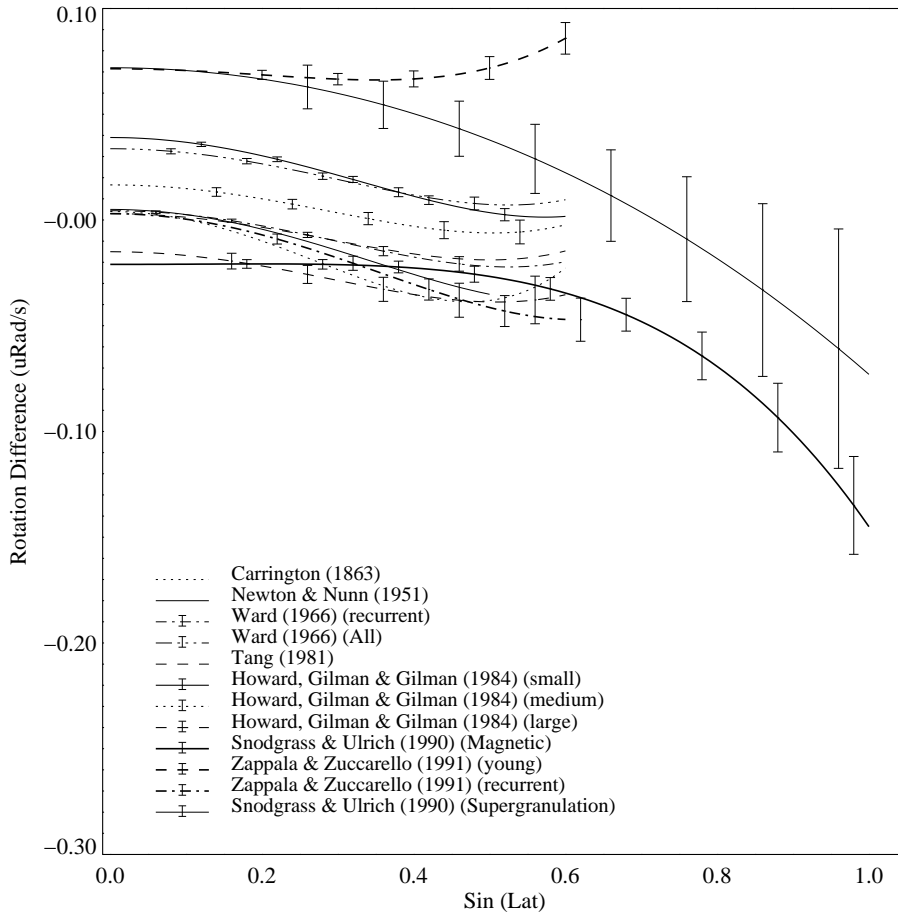
Figure 4. Tracer rotation differences. A ‘standard’ differential rotation curve ( 2.90 - 0.35(\sin^2\phi + \sin^4\phi) ) has been subtracted from plots shown in Figure 3 to better show the differences. The variation of curvature reflects the variation of the measure of differential rotation. Young sunspots and supergranulation rotation are the higher plots. The shape of the differential rotation curves for sunspots are different than the shapes of the curves from Snodgrass and Ulrich (1990) which used supergranules or all magnetic features as tracers and extended to high latitudes.
