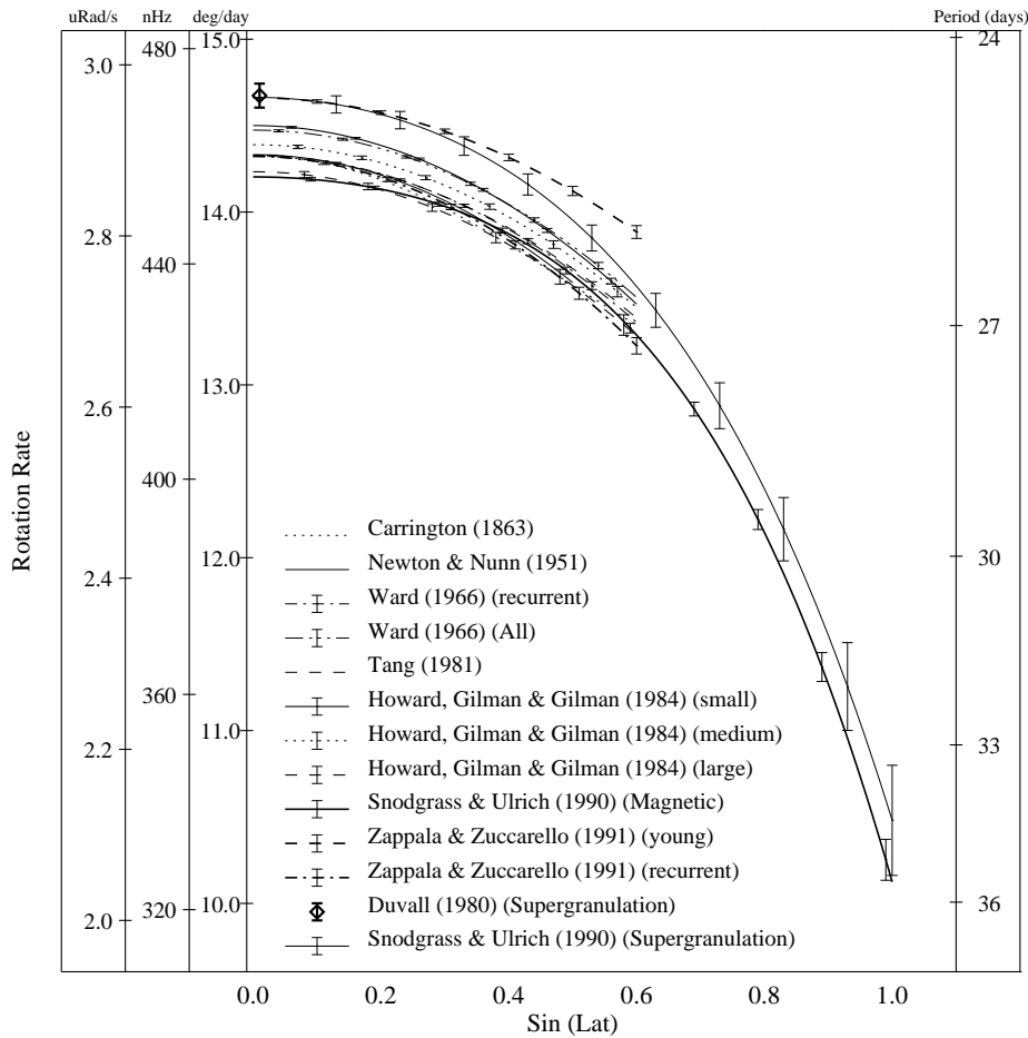
Figure 3. Tracer rotation. Measurements of differential rotation of tracers from coefficients listed in Table II. Not all curves extend to the highest latitude since few sunspots occur above 40^\circ latitude. The two curves extending to high latitudes are the magnetic field and supergranulation rotation curves from Snodgrass and Ulrich (1990). The highest rotation rates are for supergranulation and young sunspots. Recurrent and larger sunspots have lower rotation rates.
