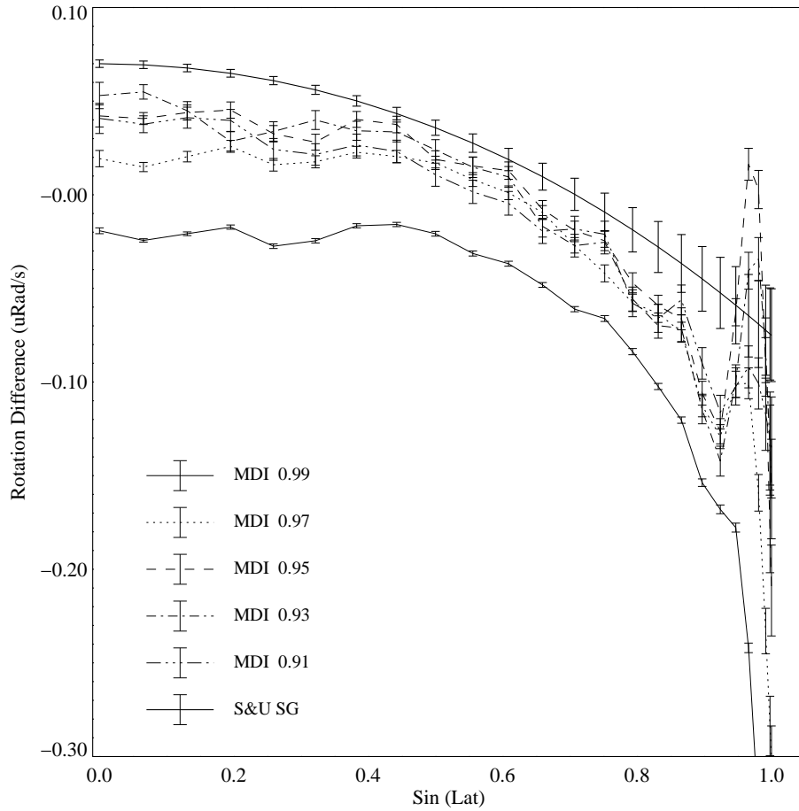
Figure 10. Differences of rotation inversions with supergranule rotations. A ‘standard’ differential rotation curve ( 2.90 - 0.35(\sin^2\phi + \sin^4\phi) ) has been subtracted from curves plotted in Figure 9 to better show the differences. The supergranulation rotation rate is clearly significantly higher than the rotation rates within the convection zone at low latitudes. At higher latitudes there is very little overlap of error bars.
