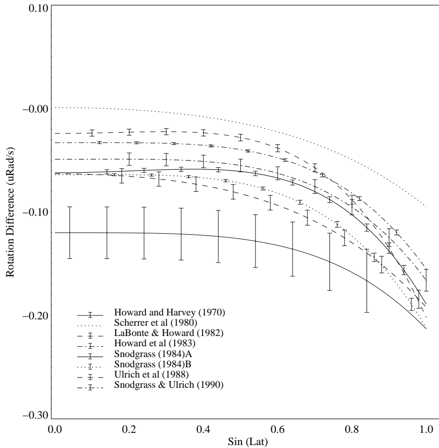
Figure 2. Spectroscopic rotation differences. A ‘standard’ differential rotation curve ( 2.90 - 0.35(\sin^2\phi + \sin^4\phi) ) has been subtracted from curves plotted in Figure 1 to better show the differences. The variation of curvature reflects the variation of the measure of differential rotation. The plots of Howard et al. (1983), Snodgrass (1984) B and Snodgrass and Ulrich (1990) show the most similar differential rotation curve; although the absolute rates of rotation are quite different between these three. Note that few of these measurements are consistent within error bars.
